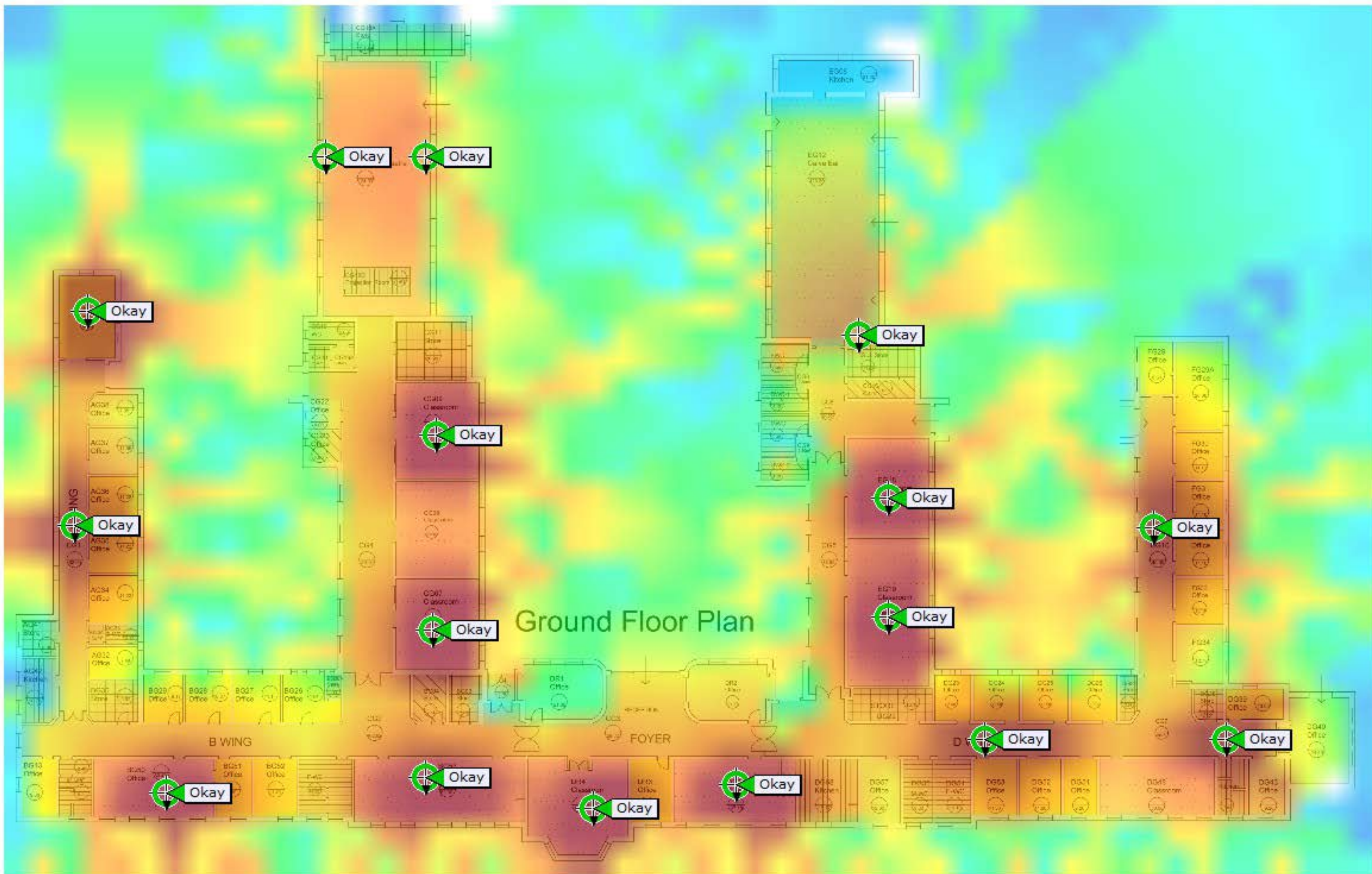
Carlisle, Fusehill Street, Calva, Ground Floor
